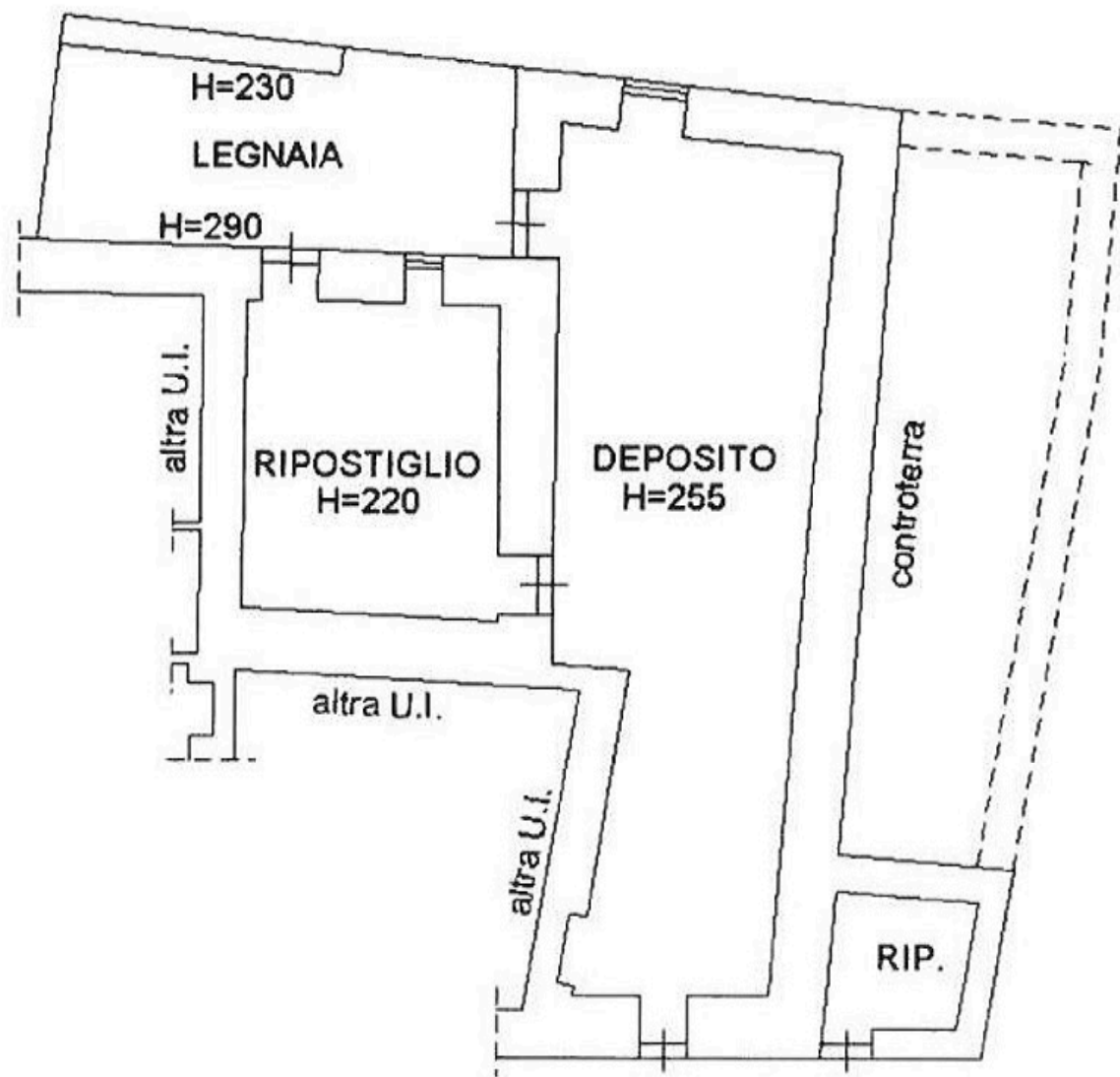
PIANO TERRA
